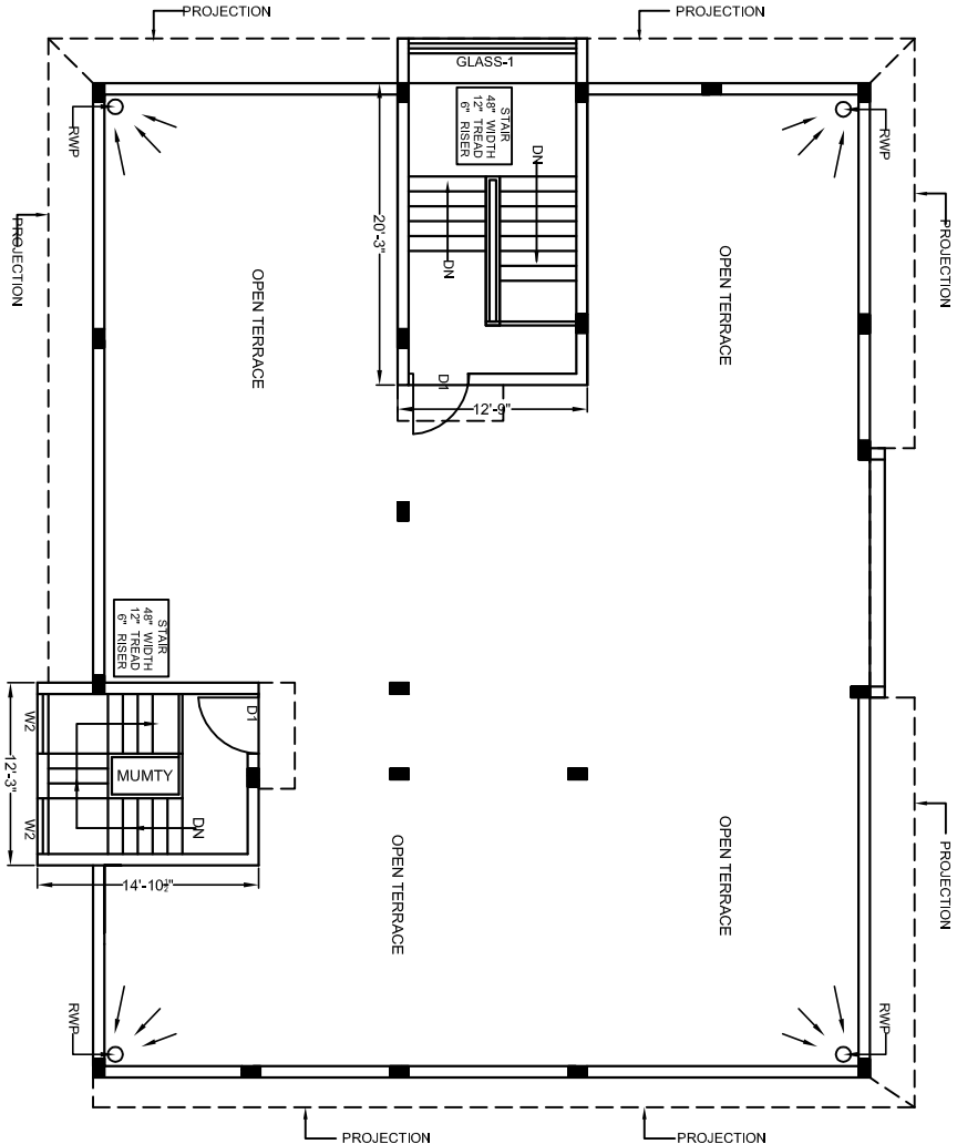
TERRACE PLAN
