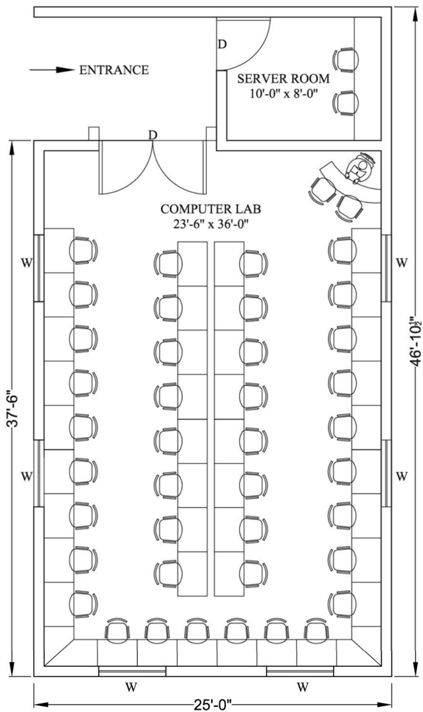
LAYOUT PLAN OF COMPUTER LAB AT GOVT.GIRLS INTER COLLEGE RAJPUR ROAD DEHRADUN
